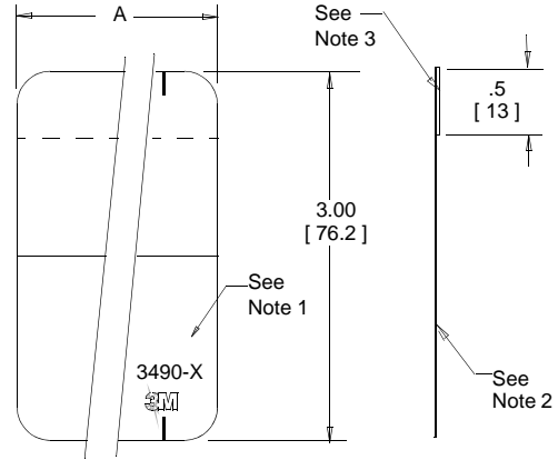
Standard Pull Tab 3490
